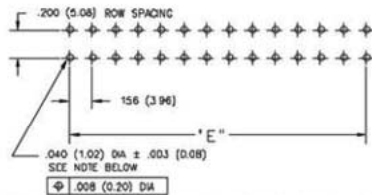
RECOMMENDED MOTHER BOARD HOLE PATTERN
